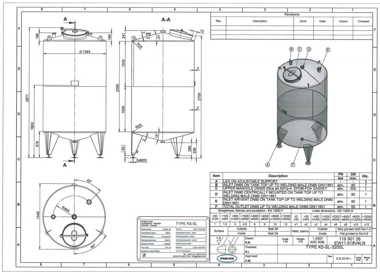
Technical drawing
